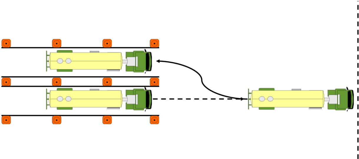
Figure 11.3: Offset Back/Left
