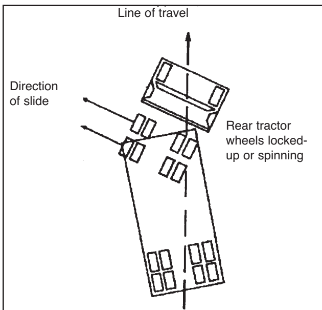
Figure 6-2--Tractor Jackknife
