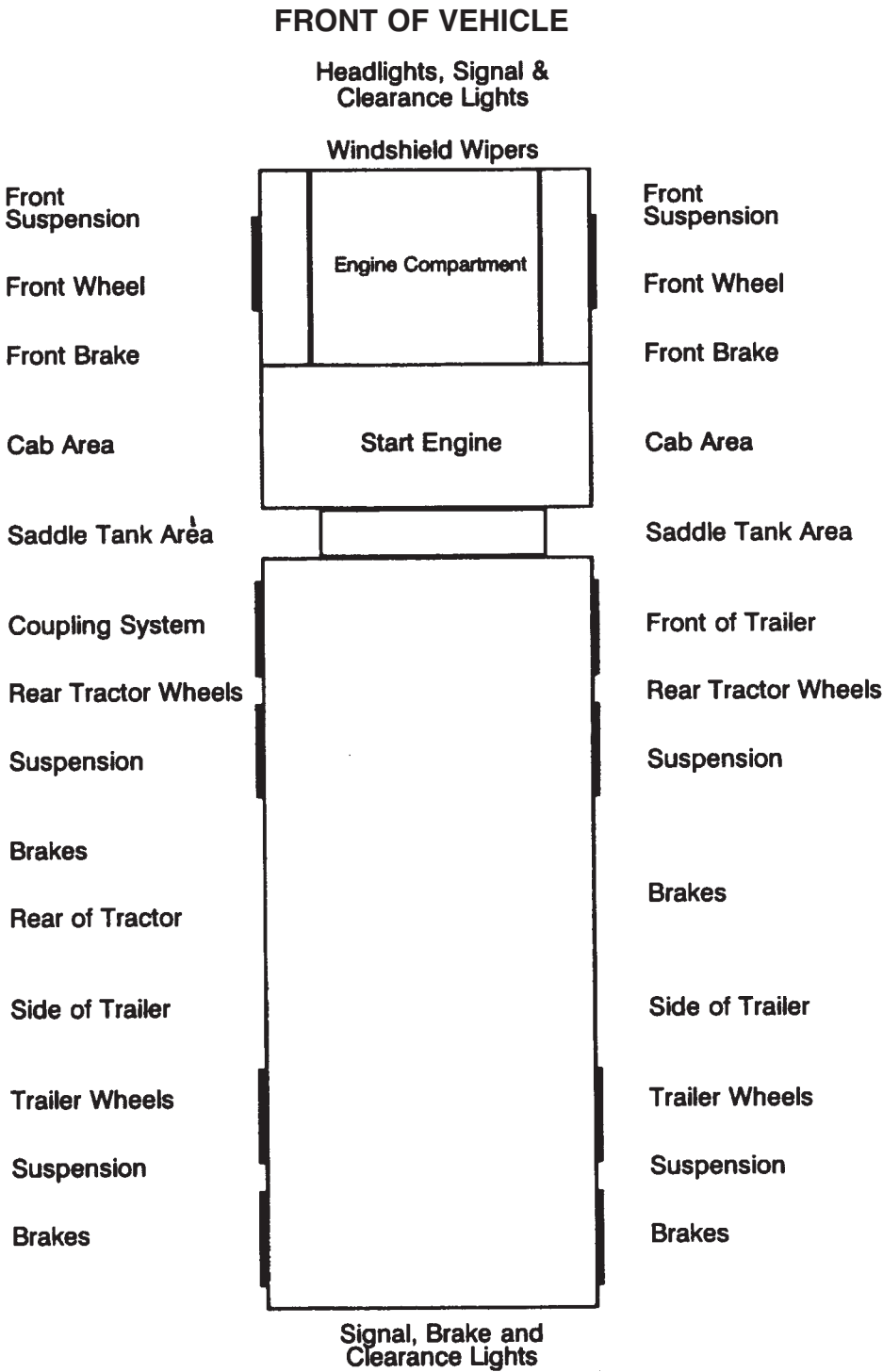
Figure 2.7 -- Tractor-Trailer
